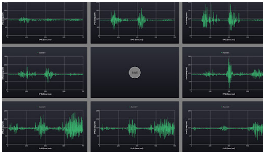
Figure 2: Example of raw EMG data from the eight channels on the EMG armband [4]
